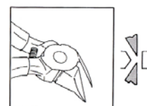
PL-756・757の刃先状態 Cutting blade (for plastic cutting pliers)
